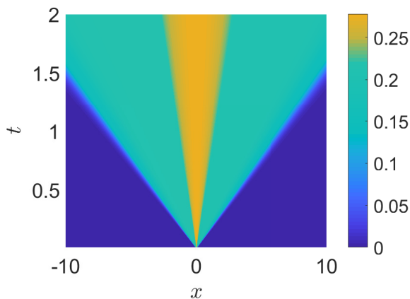
FIG. 1: The light-core diagram of the of the energy current of the 1D BF mixtures at low temperatures. The initial state is set up as two semi-infinitely long 1D tubes joined together with different temperatures.
